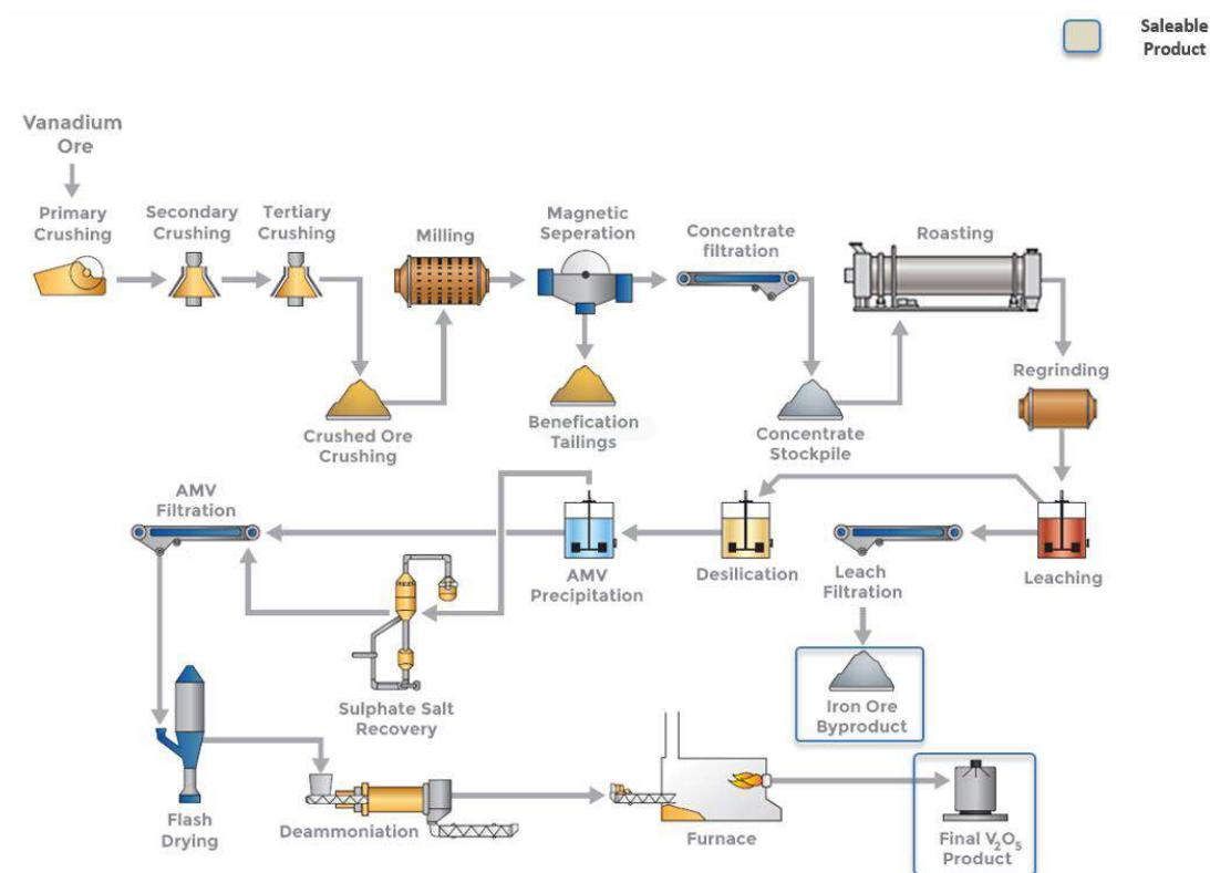
High-level illustrative block flow diagram of vanadium plant
