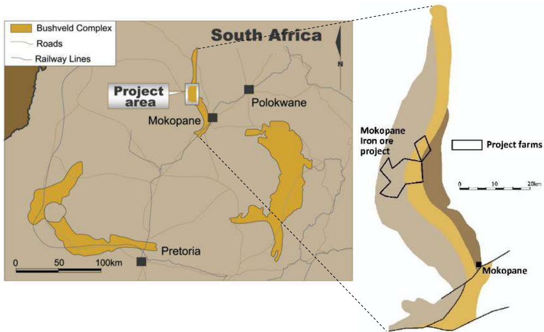
Location of the Mokopane Iron Ore Project in relation to the Bushveld Complex and infrastructure
